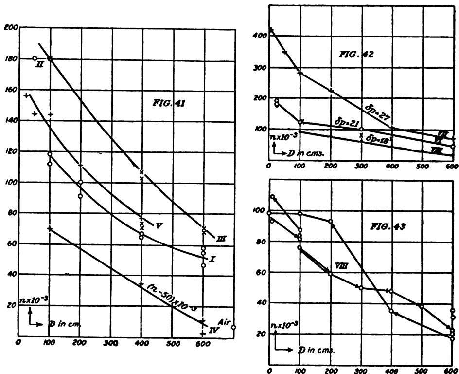
FIGS. 41, 42, and 43.—Nucleations (ions) produced by a radiating X-ray bulb at different distances ( D ) from the small wood fog chamber. Table 34.
